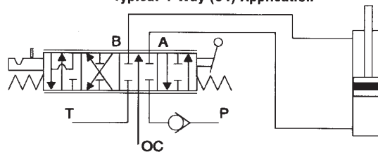
Typical 4-Way Float (K4) Application
