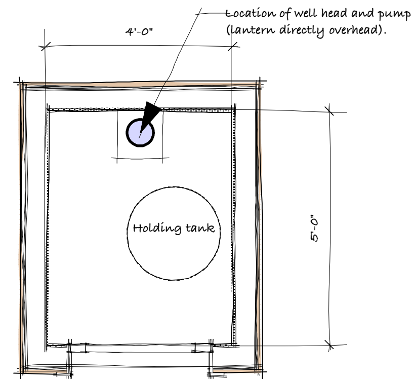
Plan
