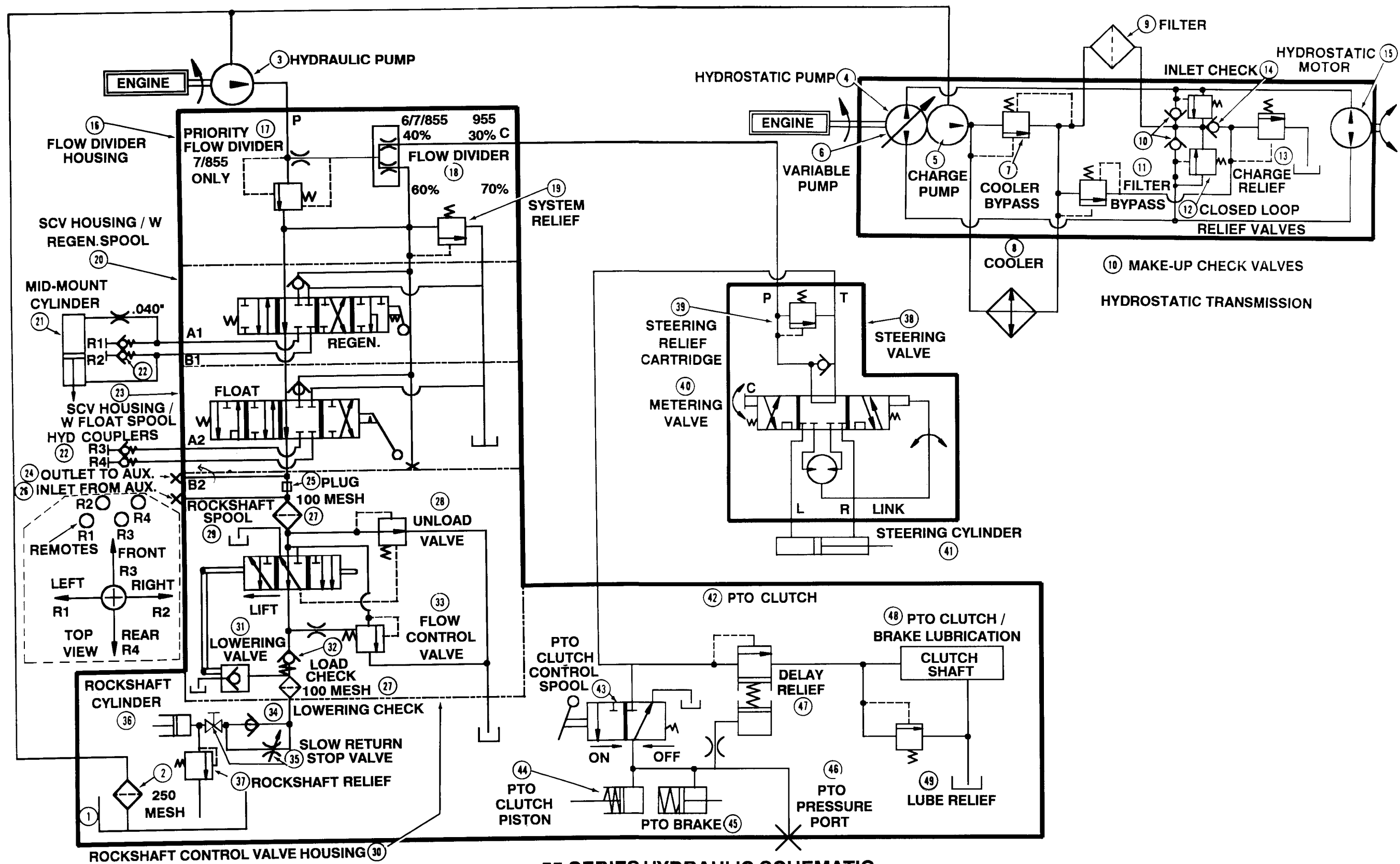
55 SERIES HYDRAULIC SCHEMATIC
