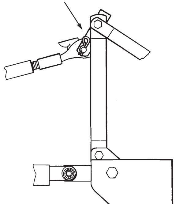
Figure 2-6 Flex-Link
